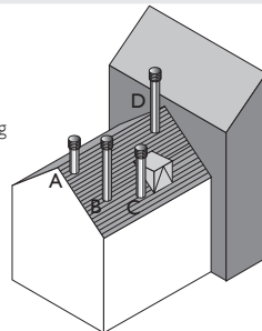
Fig. B Outlet siting for wood burning appliances (<50kw)
