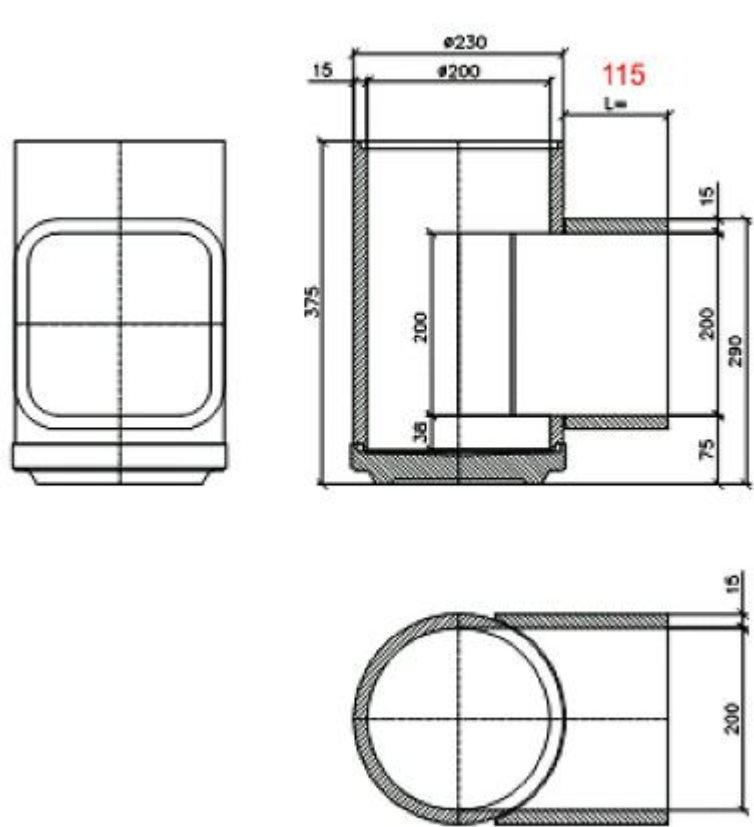
T-PIECE with bottom ceramic plate DN200
