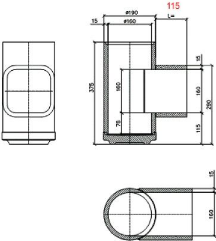
T-PIECE with bottom ceramic plate DN160
