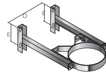
Structural Wall Band with Types L1 & L2 Extension Assembly
