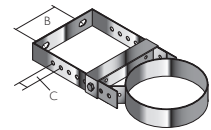
Wall Band and Adjustable Back Bracket Assembly
