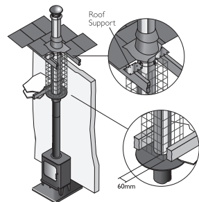
Internal Bungalow (Ventilated Loft Space) Combustible and Non-Combustible Floors
