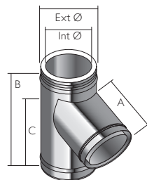
135° Tee
