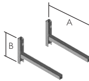
Cantilever Brackets - Types 325, 475
