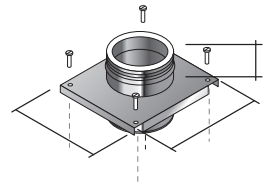
Fig.1 Top Plate
